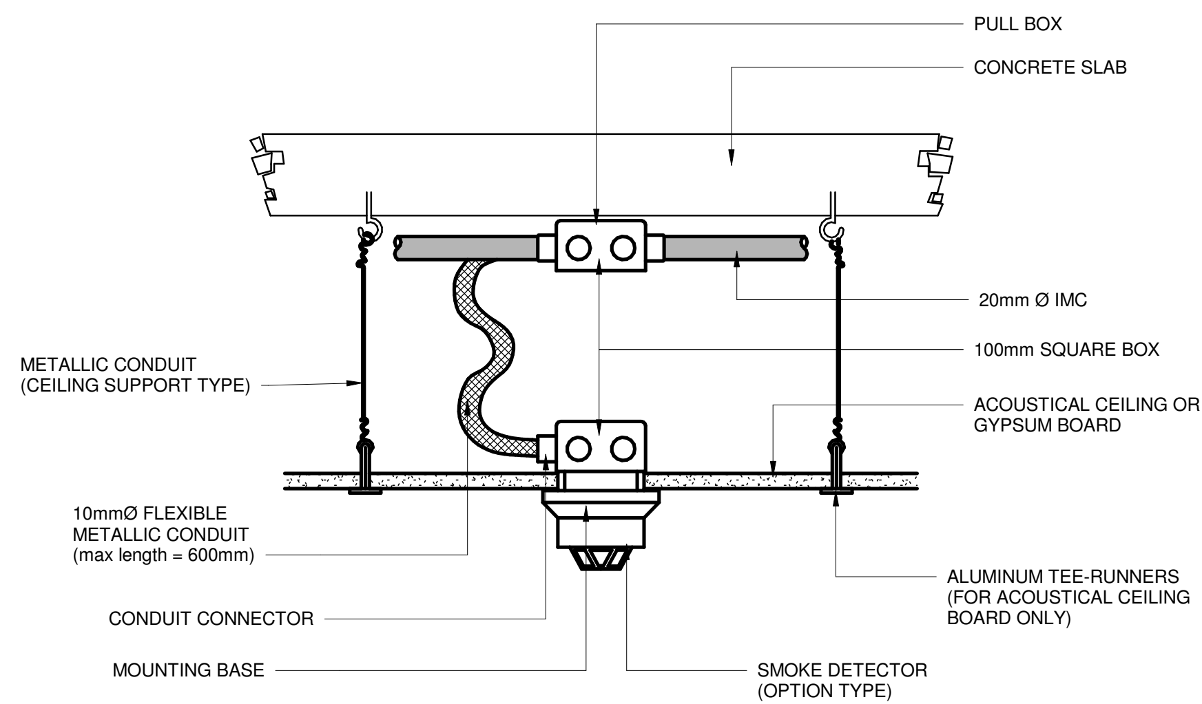
1 SMOKE DETECTOR MOUNTING DETAILS I N T S
