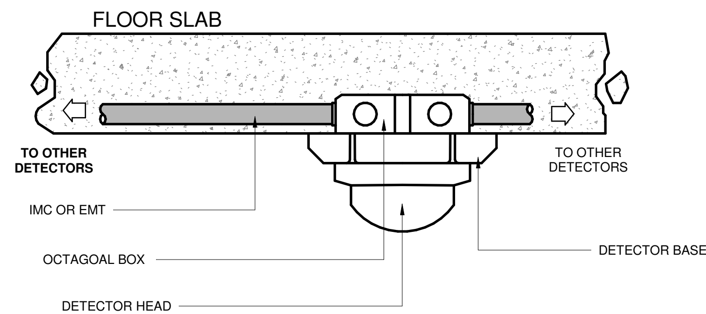
2 SMOKE DETECTOR MOUNTING DETAILS II N T S
