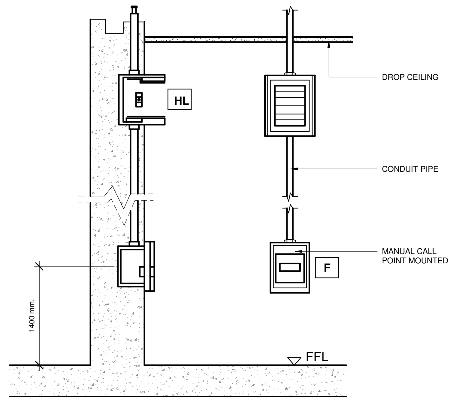
3 MOUNTED DETAIL OF MANUAL PULL STATION N T S
