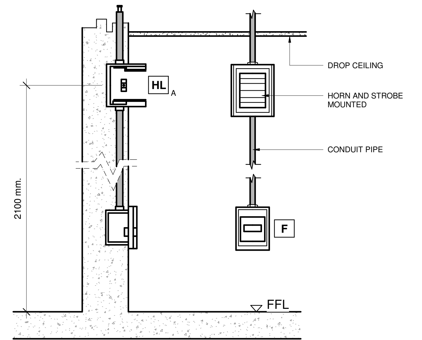
5 MOUNTED DETAIL OF HORN STROBE N T S
