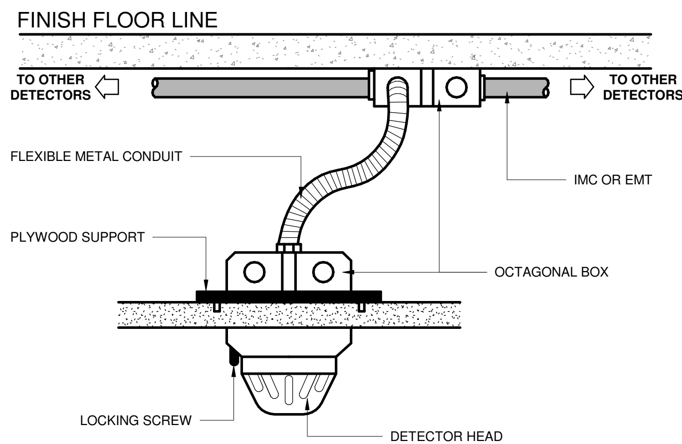
4 DETECTOR DETAIL ON DROP CEILING W/ CONDUIT EXPOSED N T S
